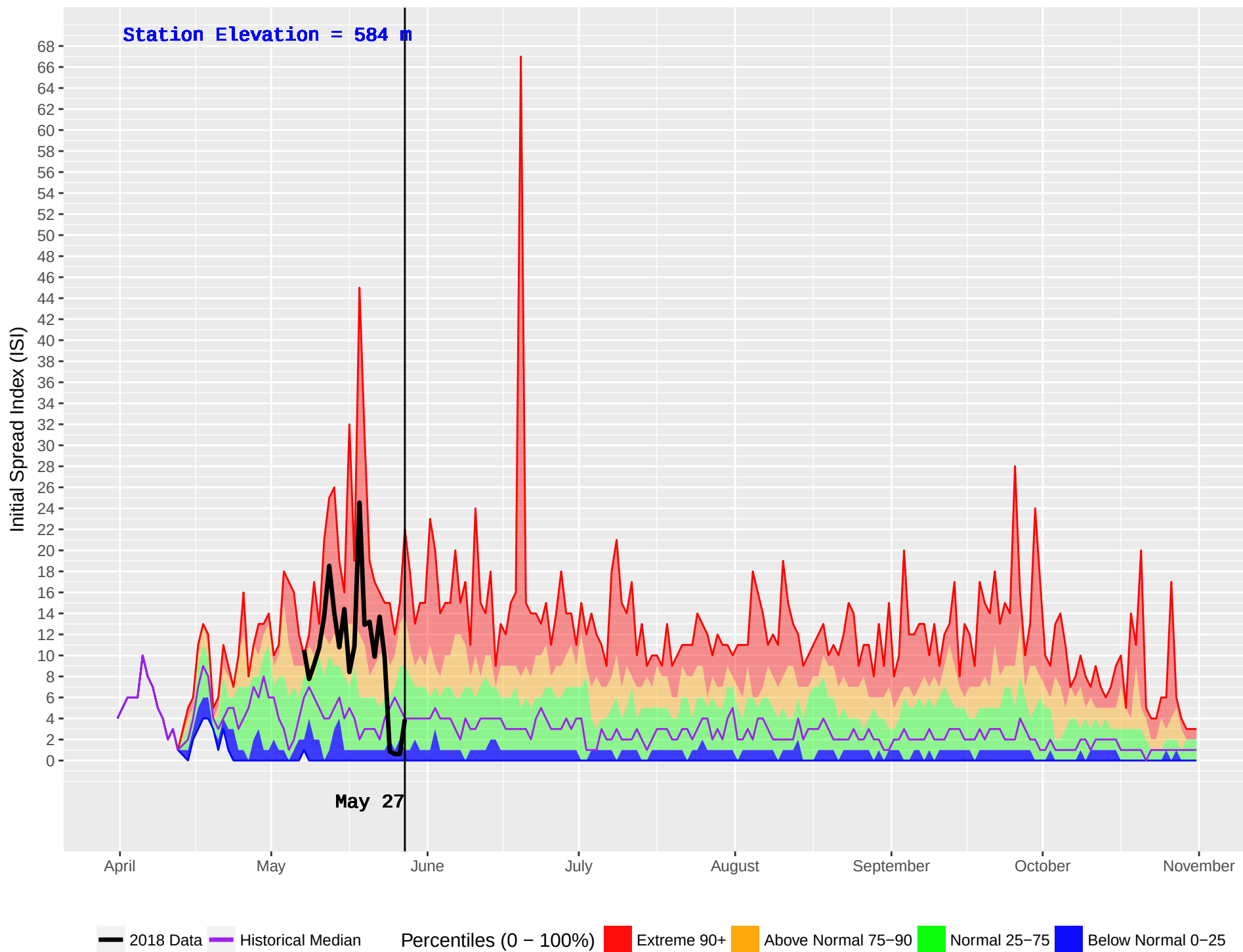
SIERRA (117) : Historical (1981–2016) and Current (2018) Noon Initial Spread Index (ISI)
