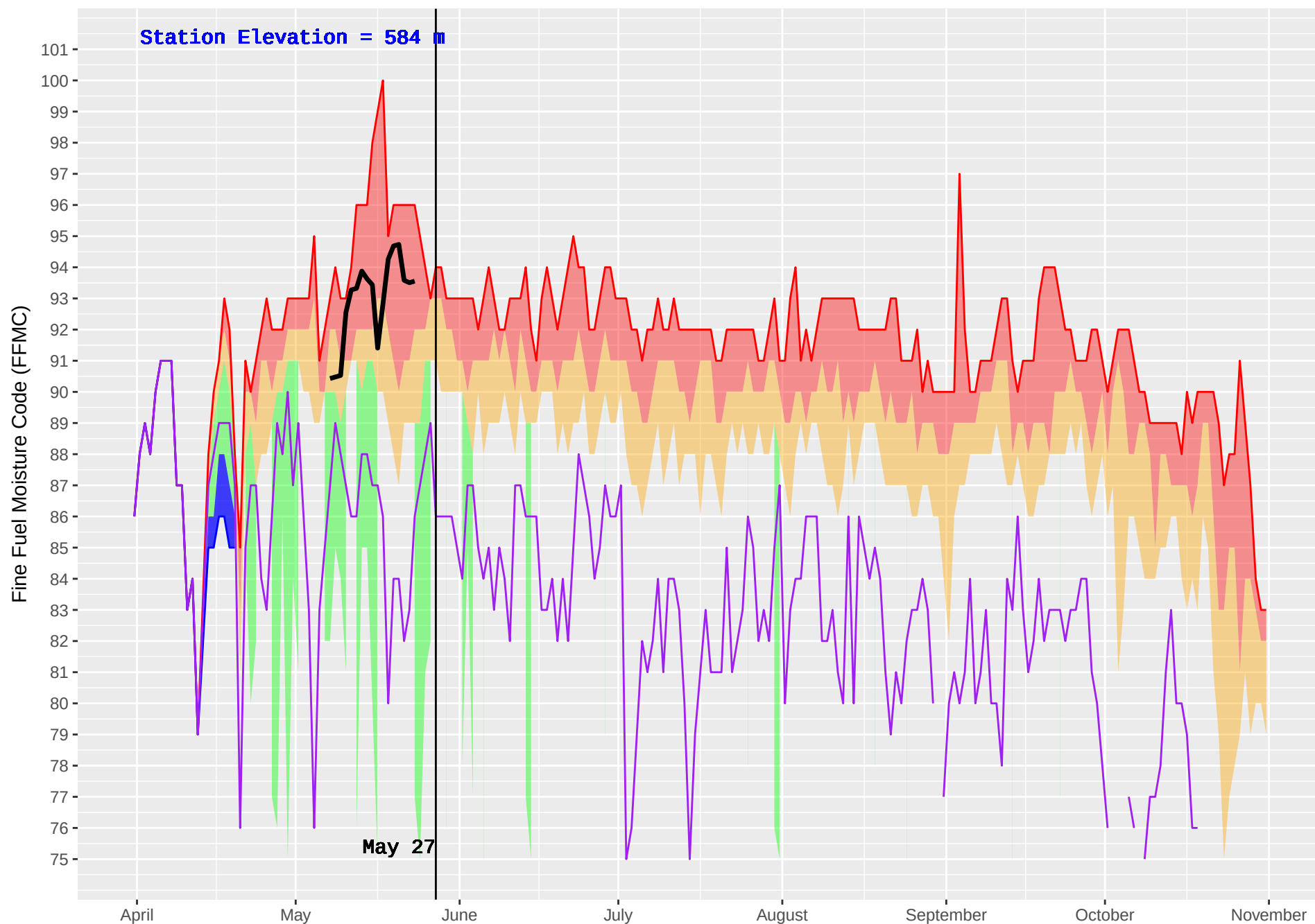
SIERRA (117) : Historical (1981–2016) and Current (2018) Noon Fine Fuel Moisture Code (FFMC)
