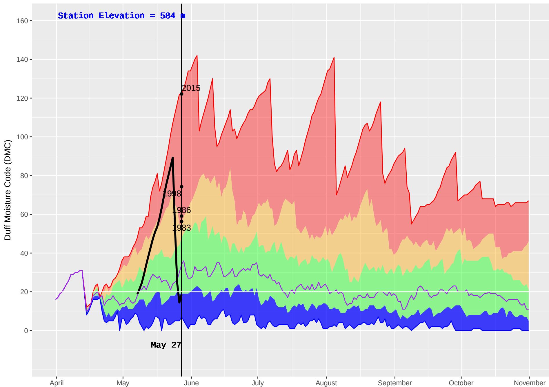
SIERRA (117) : Historical (1981–2016) and Current (2018) Noon Duff Moisture Code (DMC)
