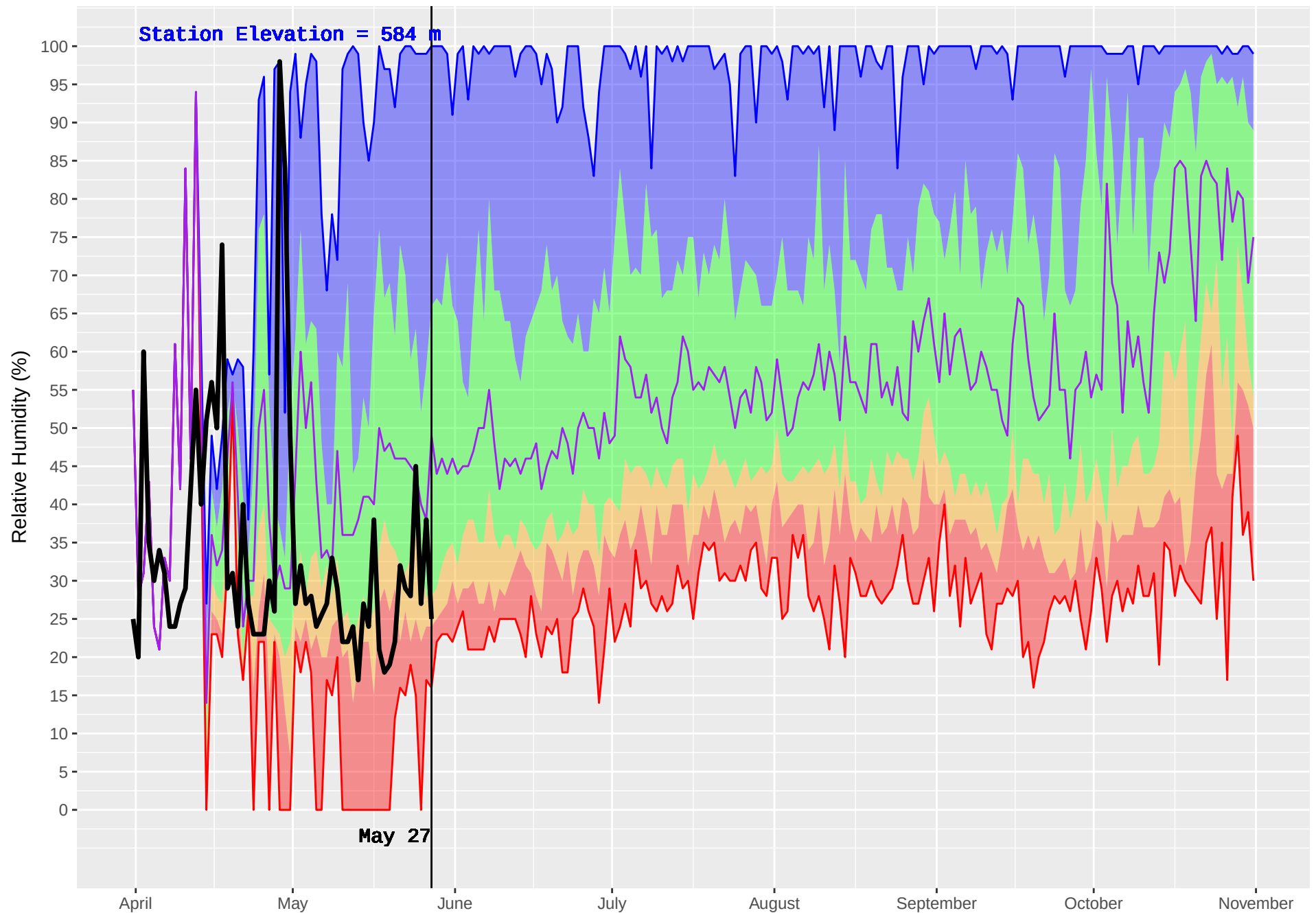
SIERRA (117) : Historical (1981–2016) and Current (2018) Noon Relative Humidity
